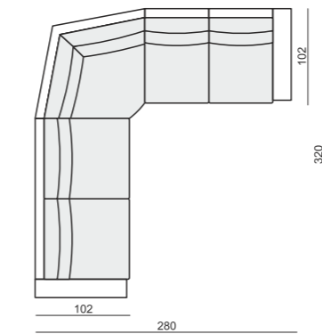
SET 13 RIGHT (or LEFT) 3 SEATER 90 LEFT (or RIGHT) + CORNER 90° + 2 SEATER 70 RIGHT (or LEFT)
