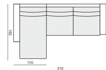
SET 16 LEFT (or RIGHT) CHAISELONGUE 90 LONG LEFT (or RIGHT) + 3 SEATER 90 RIGHT (or LEFT)
