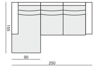
SET 1 LEFT (or RIGHT) CHAISELONGUE 70 LEFT (or RIGHT) + 2 SEATER 70 RIGHT (or LEFT)
