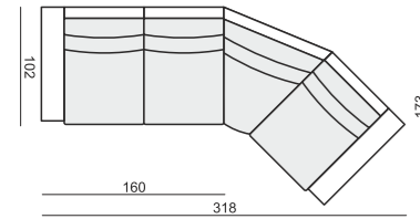
SET 3 RIGHT (or LEFT) 2 SEATER 70 LEFT (or RIGHT) + CORNER 45° + ARMCHAIR 70 RIGHT (or LEFT)
