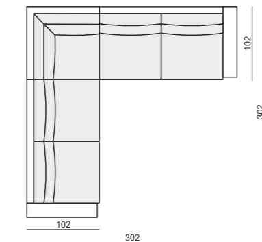
SET 8 3 SEATER 90 LEFT + CORNER 90° + 3 SEATER 90 RIGHT
